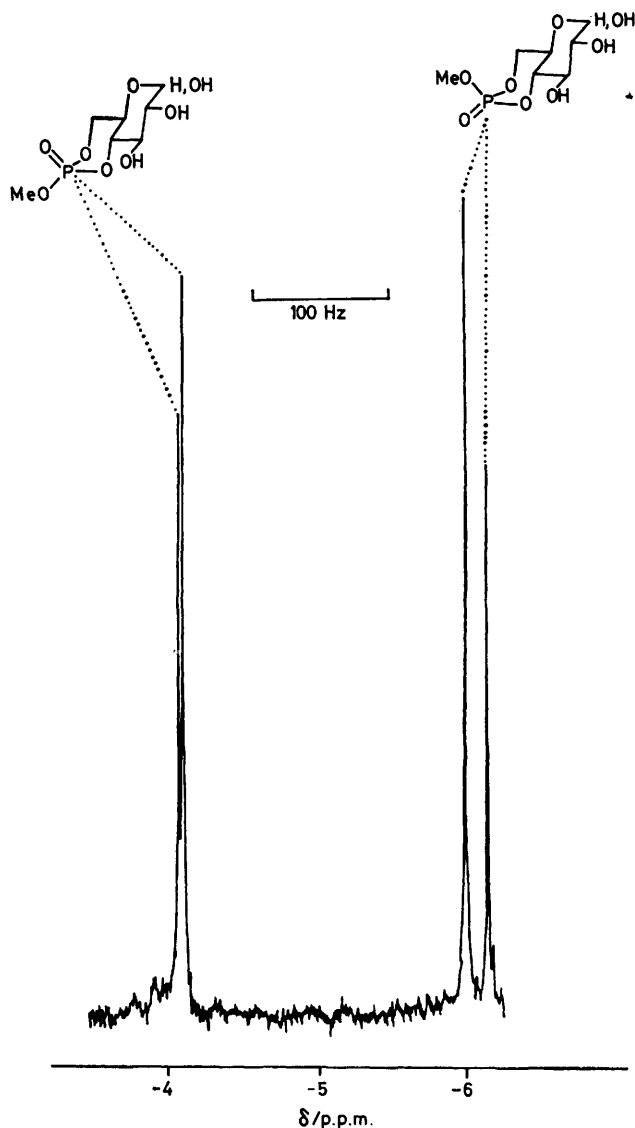
FIGURE 1 The ^{31}\text{P} n.m.r. spectrum (121.5 MHz) of the \alpha - and \beta -anomers of the axial and equatorial methyl esters of D-glucose 4,6-phosphate in 25% \text{CD}_3\text{OD} , 75% MeOH containing 8-hydroxyquinoline. Parameters: Offset 2 240 Hz, sweep width 2 000 Hz, acquisition time 2.05 s, pulse width 16 \mu\text{s} , broadband proton decoupling, line broadening 0.2 Hz in 8 K and Fourier transform in 32 K
