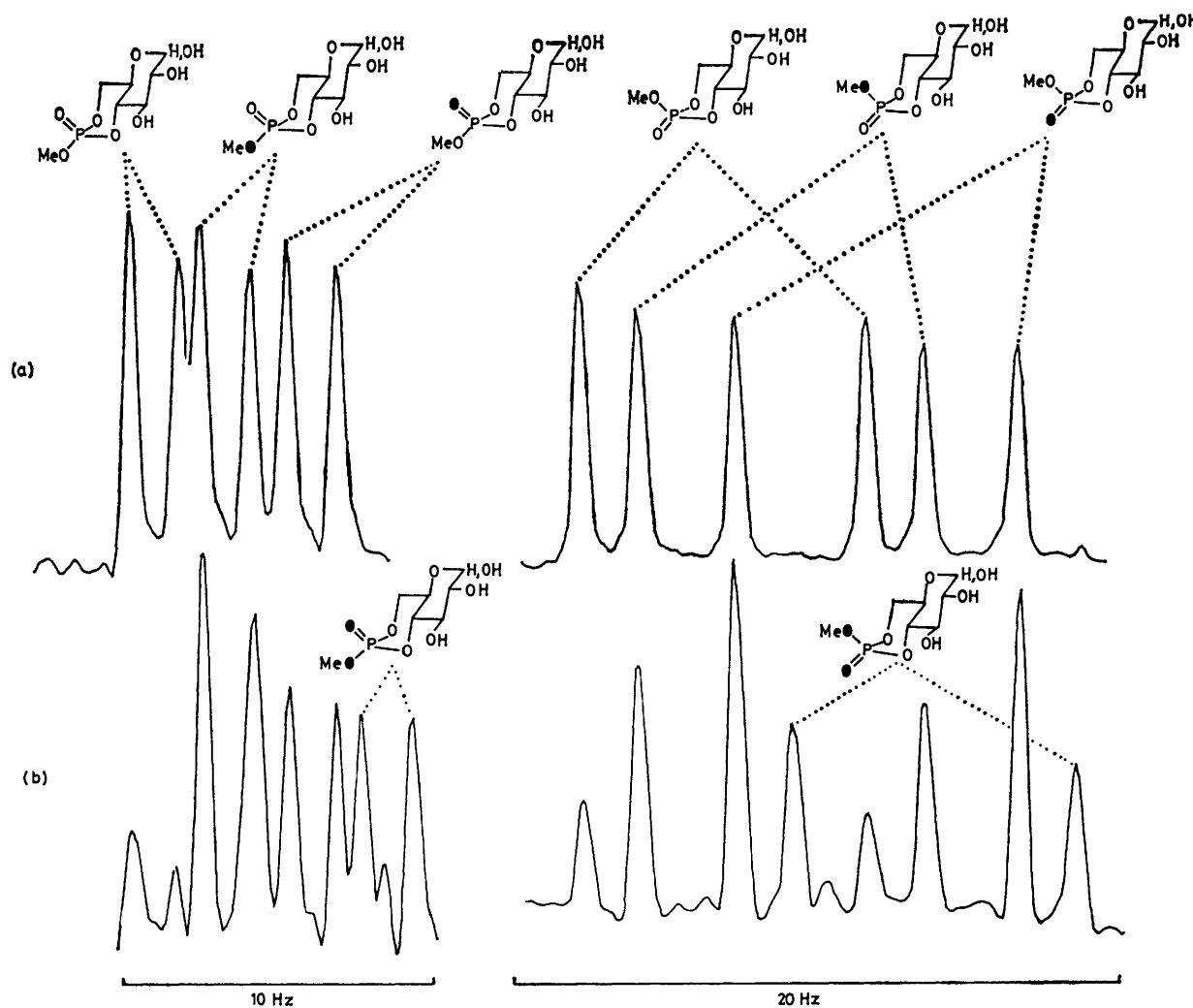
FIGURE 3 The ^{31}\text{P} n.m.r. spectra (121.5 MHz) of the axial and equatorial triesters (in 25% \text{CD}_3\text{OD} , 25% \text{MeOH} , 50% \text{Me}_2\text{SO} ) obtained by cyclisation and esterification of (a) D-glucose 6- ^{18}\text{O} ]phosphate and (b) D-glucose 6- [(S)\text{-}^{16}\text{O}, ^{17}\text{O}, ^{18}\text{O}] phosphate as shown in Scheme 4. Parameters: offset 2 240 Hz, sweep width 2 000 Hz, acquisition time 2.05 s, pulse width 16 \mu\text{s} , broadband proton decoupling, gaussian multiplication (line broadening -0.6 Hz, gaussian broadening 0.4) in 8 K, and Fourier transform in 32 K. The gain control for the equatorial triester is four times that for the axial ester in (a) and sixteen times that for the axial triester in (b)
