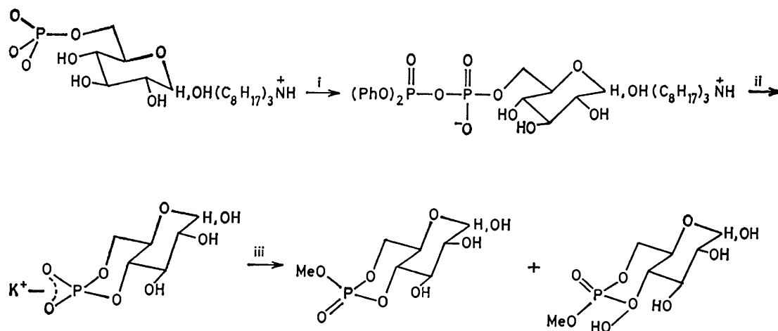
SCHEME 4 Reagents: (i) (\text{PhO})_2\text{POCl} , \text{Bu}_3\text{N}_3^+ in dioxan; (ii) \text{Bu}^4\text{OK} in \text{Me}_2\text{N}\cdot\text{CHO} ; (iii) 18-crown-6, MeI in \text{Me}_2\text{SO}
