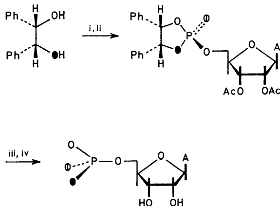
SCHEME 3 Reagents: (i) \text{P}^{17}\text{OCl}_3 , \text{C}_5\text{H}_5\text{N} ; (ii) 2',3'-diacetyl-adenosine, \text{C}_5\text{H}_5\text{N} ; (iii) \text{H}_2 , Pd; (iv) \text{NH}_3 , EtOH
