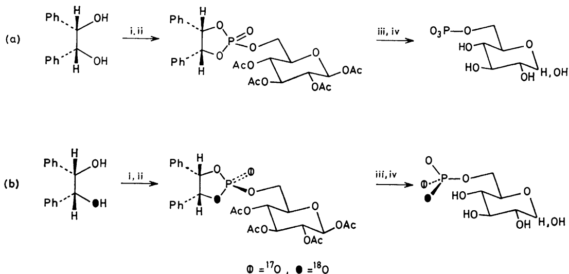
SCHEME 2 Reagents: (i) \text{C}_5\text{H}_5\text{N} , (a) \text{POCl}_3 or (b) \text{P}^{17}\text{OCl}_3 ; (ii) 1,2,3,4-tetra-acetyl- \beta -D-glucose, \text{C}_5\text{H}_5\text{N} ; (iii) \text{H}_2 , Pd; (iv) KOMe, MeOH
