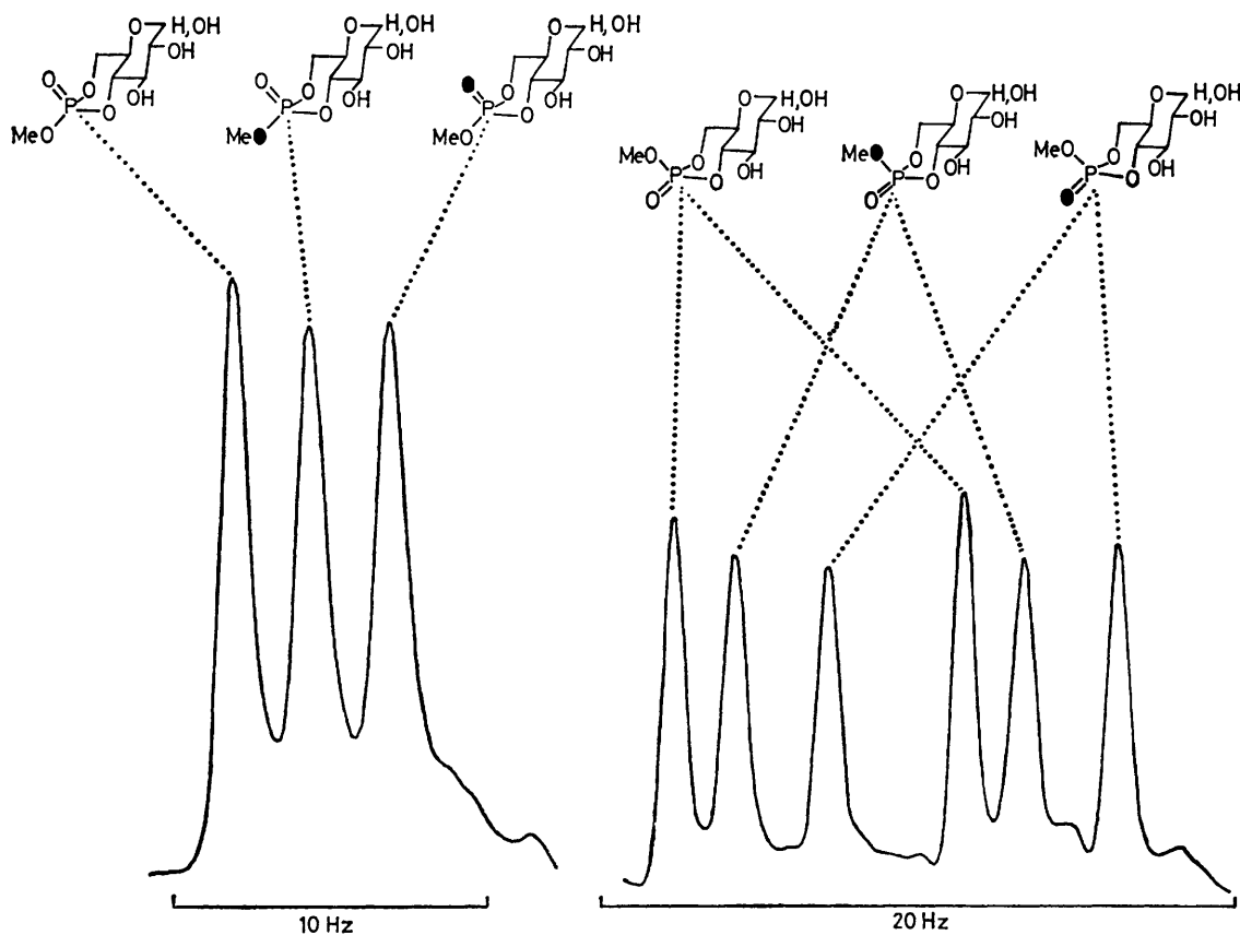
FIGURE 2 The ^{31}\text{P} n.m.r. spectrum (121.5 MHz) of the axial and equatorial triesters (in \text{CD}_3\text{OD} ) obtained by cyclisation and esterification of D-glucose 6- ^{18}\text{O} phosphate using dicyclohexylcarbodi-imide in pyridine. Parameters: offset 2 649 Hz, sweep width 1 202 Hz, acquisition time 2.05 s, pulse width 16\ \mu\text{s} , broadband proton decoupling, gaussian multiplication (line broadening -1.0 Hz, gaussian broadening 0.1) in 4 K and Fourier transform in 32 K
