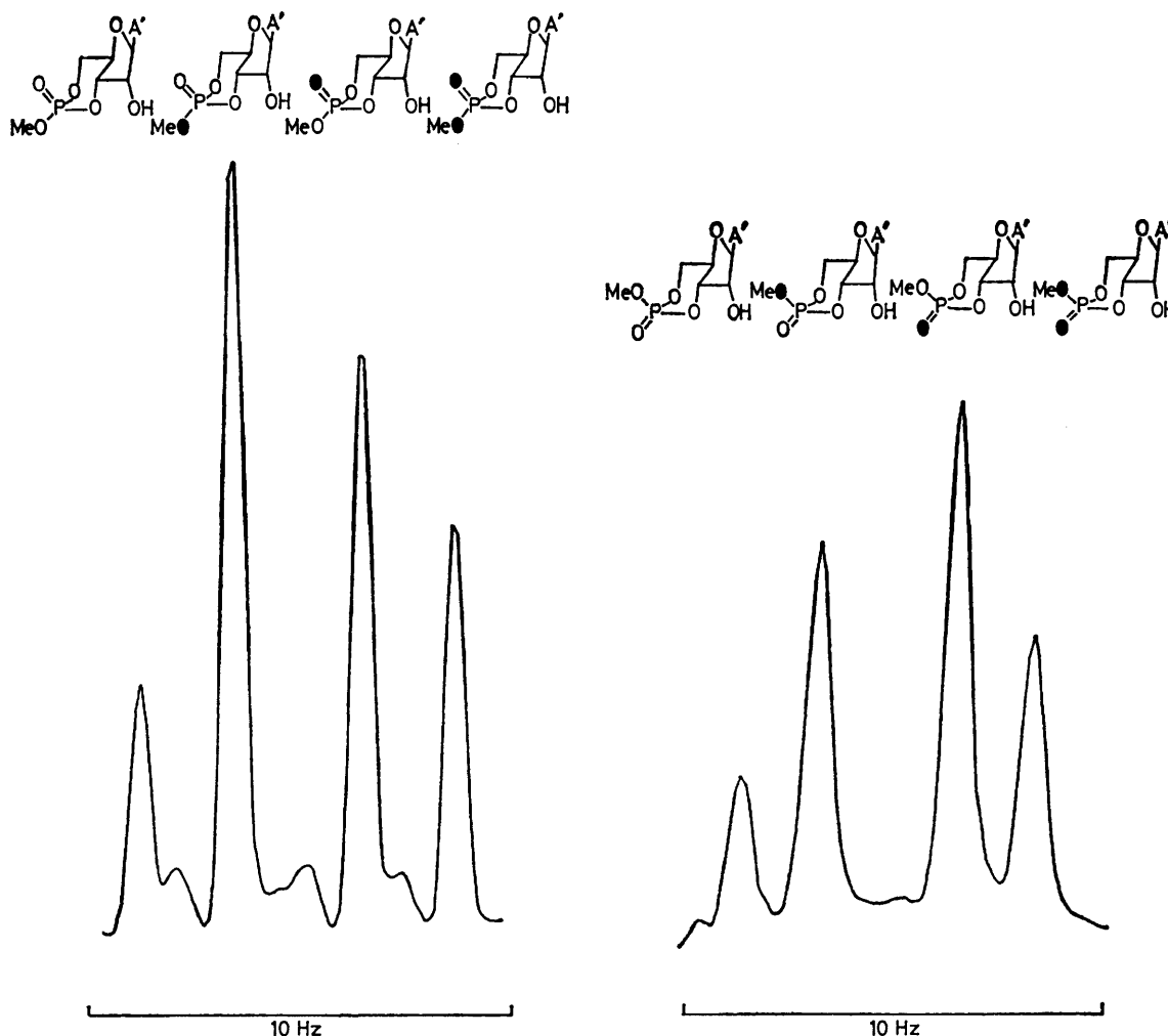
FIGURE 4 The ^{31}\text{P} n.m.r. spectrum (121.5 MHz) of the axial and equatorial triesters (in 1:1 \text{Me}_2\text{SO}-(\text{CD}_3)_2\text{SO} ) derived by cyclisation (with diphenyl phosphorochloridate followed by potassium t -butoxide) and esterification of adenosine 5'-[( S )- ^{18}\text{O} , ^{17}\text{O} - ^{18}\text{O} ]phosphate. Parameters are similar to those in Figure 3. The gain control for the equatorial triester is twice that of the axial triester. A' = N -1-methyladenine
